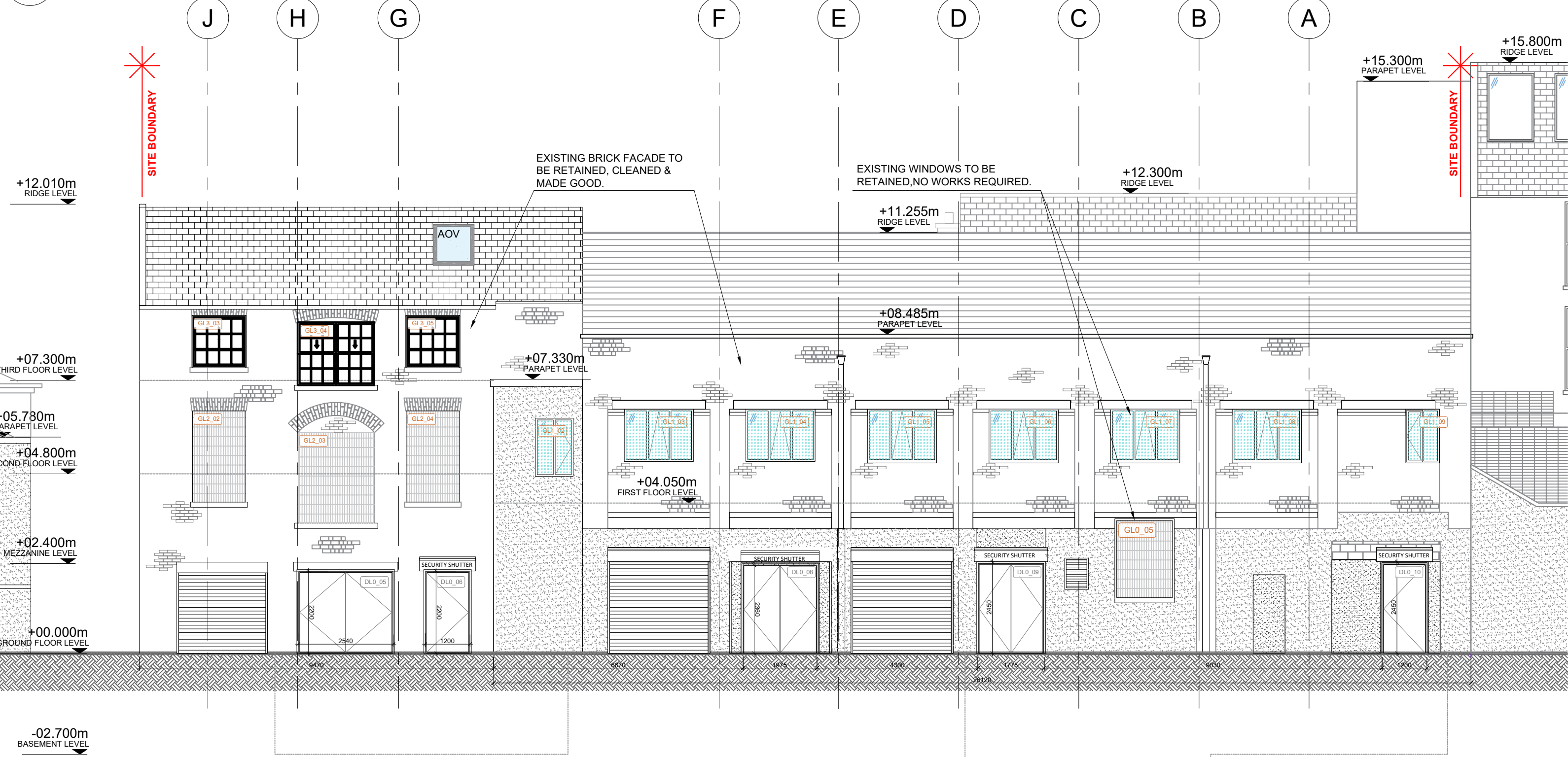
2 30.10 SOUTH ELEVATION_MARLBOROUGH PLACE SCALE: 1:100
